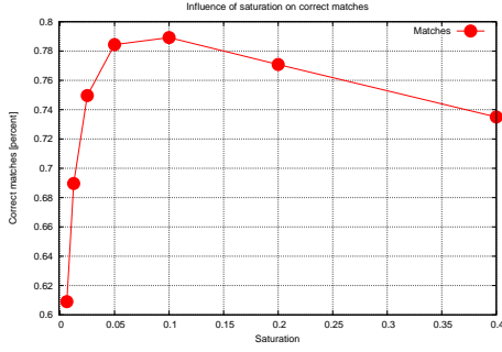
Fig. 3. Influence of saturation on correct matches.
