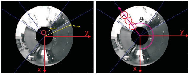
Fig. 1. Extraction of the most reliable vertical features.
