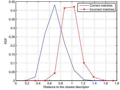
Fig. 6. The probability density function that a match is correct according to the first rule.
