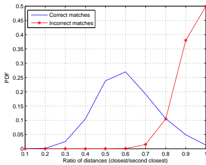
Fig. 8. The probability density function that a match is correct according to the third rule.
