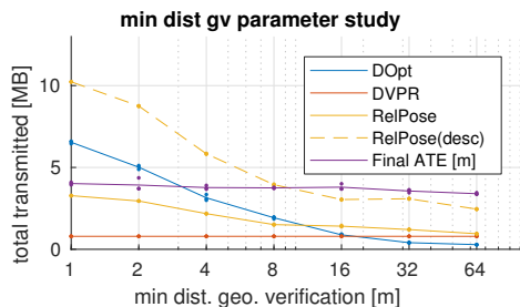
Fig. 8. Effect of changing \tau_{\text{mdg}} , the parameter that controls the distance between an established relative pose \tilde{z}_{\beta_j}^{\alpha_i} and the next frame of \alpha to be sent to \beta for geometrical verification. As we can see, \tau_{\text{mdg}} can be used to significantly throttle the required bandwidth. This happens without a significant effect on the ATE. The dashed line indicates RelPose data transmission if descriptors are used for keypoint association rather than visual word indices.
