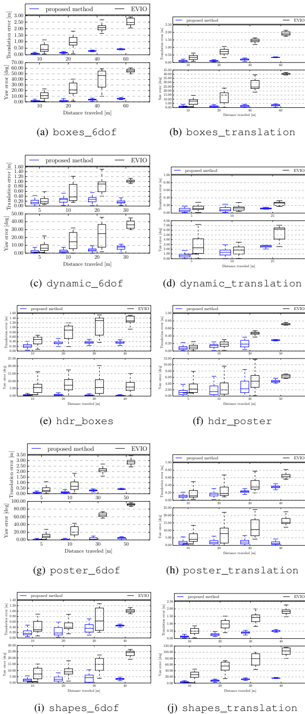
Figure 1: Detailed comparison of our proposed method against EVIO on the Event Camera Dataset.
